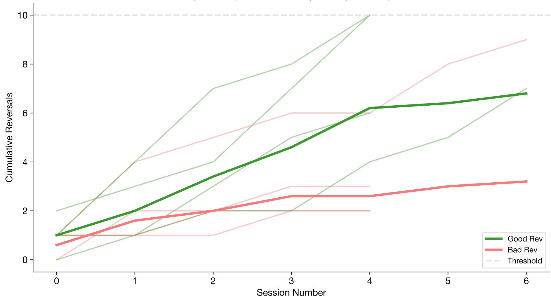
Cumulative Good and Bad Reversals Over Time (n=5 subjects; sessions per subject=1-7)
